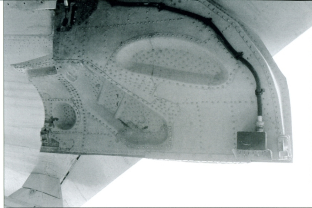
The port main wheel door of an early-production Su-27 Flanker-B has the inner surfaces painted Gray. The port main wheel door has a sensor with a cable mounted on the lower part of the door. The starboard door does not have a cable.
