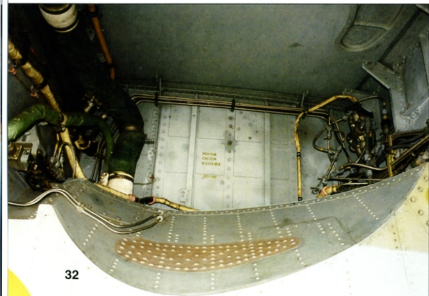
(Below) The upper port main wheel well has a number of reinforcement struts. (Jozef And'al)
