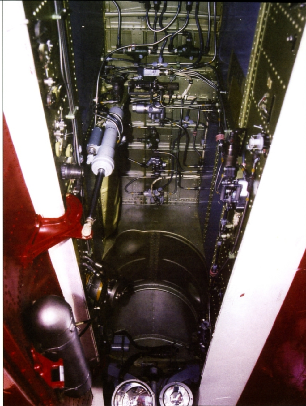
The refueling point in the nose wheel well of late-production Su-27s is one of four on the later Flanker-Bs. Three others are on the upper rear of the fuselage. Early Su-27s did not have the refueling point in the wheel well. The Su-27 has four fuel tanks, which can hold a total of 3,163 U.S. gallons (11,975 L) of T-1 or TS-1 kerosene. (Marcus Fülber)
