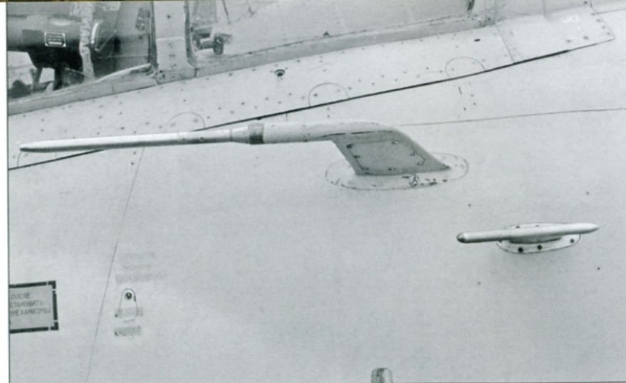
Two PVD-7 pitot tubes are located on the port side of the Su-27 Flanker-B.
