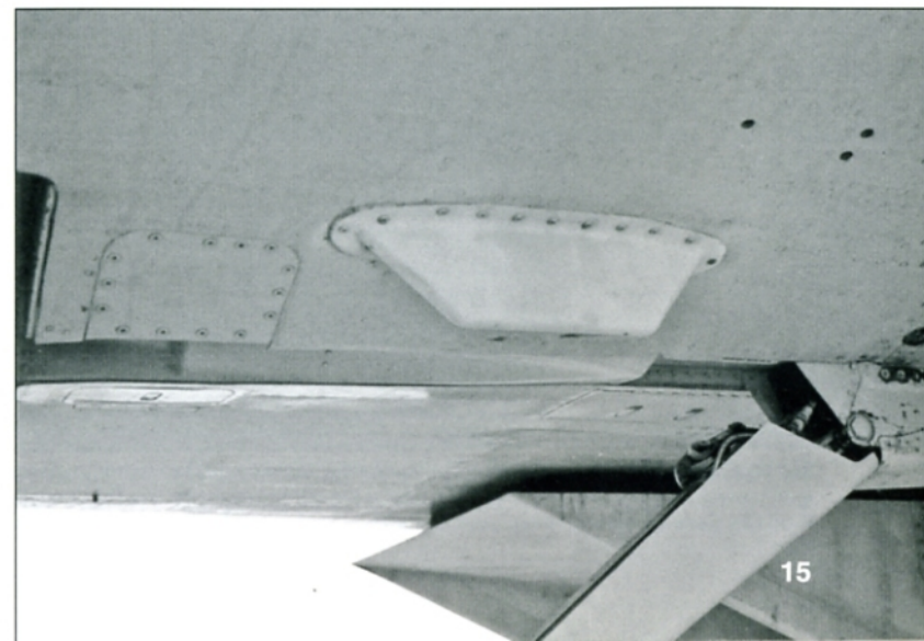
(Below) An antenna fairing is located on the port side of the nose gear extension. This antenna fairing is painted White on standard-production Su-27s but is painted Radome Green on some early-production Su-27s.
