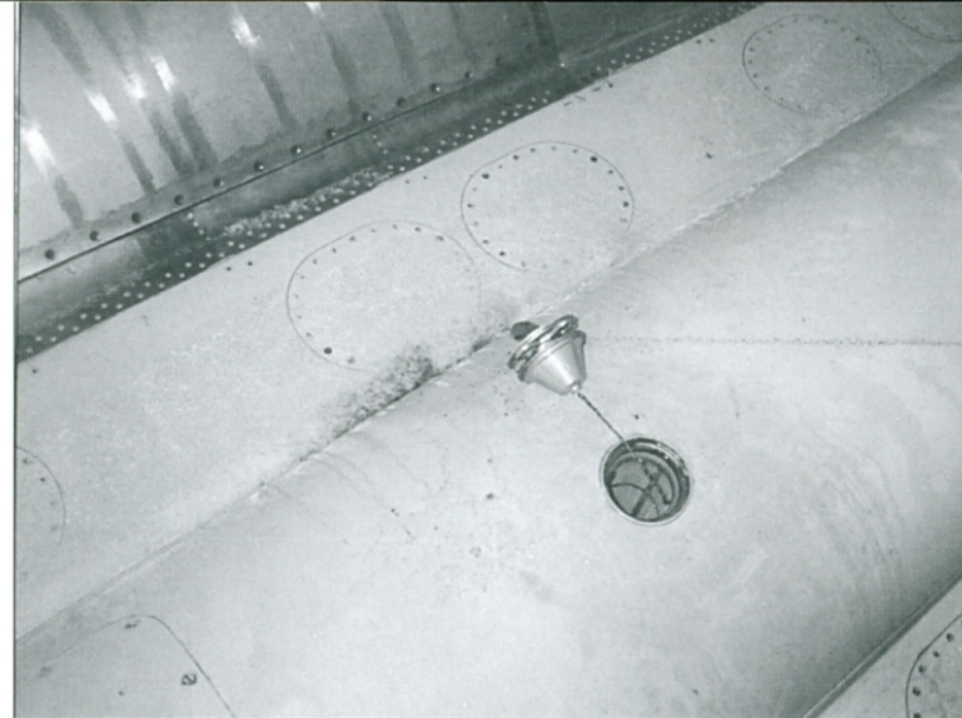
The rear fuel tank filler is located on the tail section of the Su-27 Flanker-B. The fuel tank fill services tank No. 3, the rear fuselage fuel tank, with a capacity of just more than 356 gallons (1,350 liters). The fuel tank filler on the rear fuselage was also used to drain the tanks. ( Sergej F. Sergejev )
