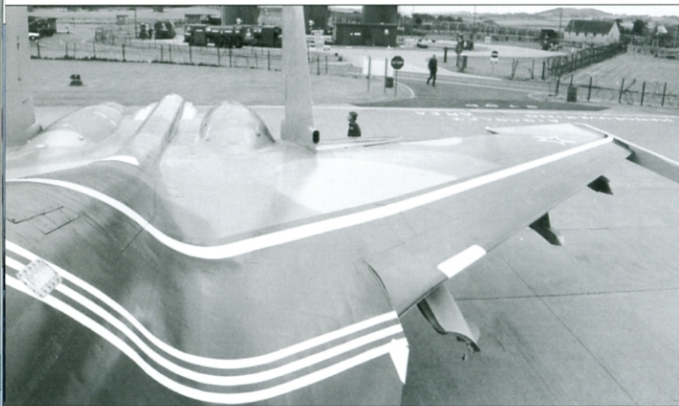
A distinctive feature of Su-27UB trainers is the White rectangular antenna on the leading-edge wing flap. Single-seat Su-27 Flankers do not have this antenna on the leading-edge wing flap. The deeper dorsal spine is also typical of the two-seat trainer. (Simon Watson)
