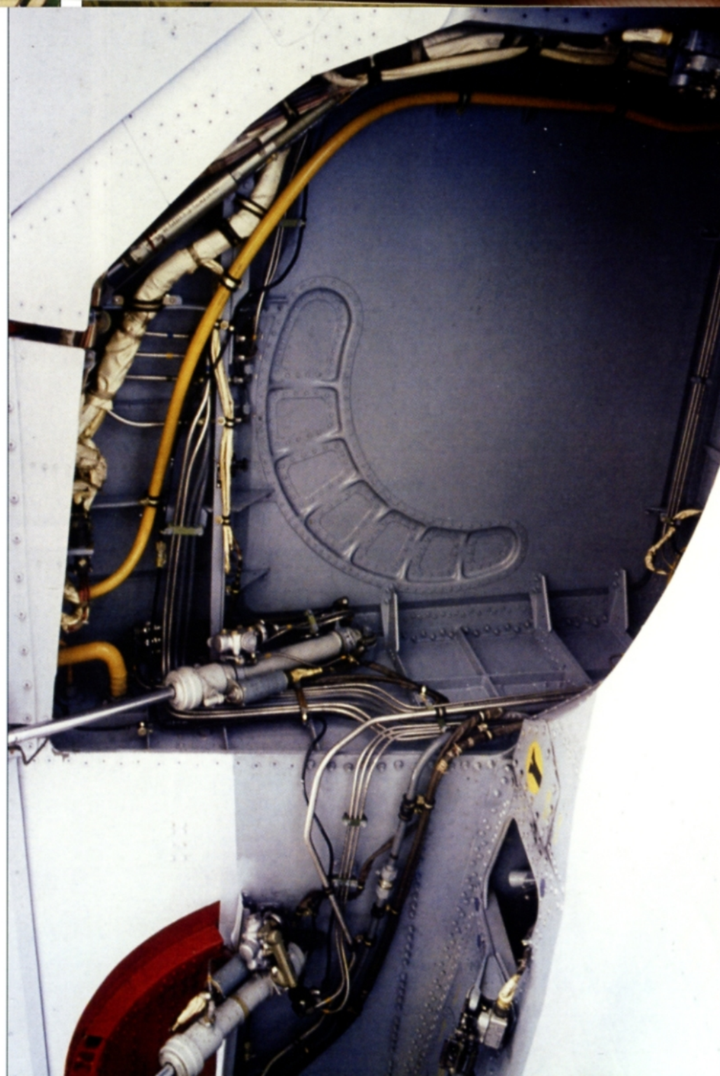
(Below) The upper port main wheel well has a number of reinforcement struts. (Jozef And'al)
