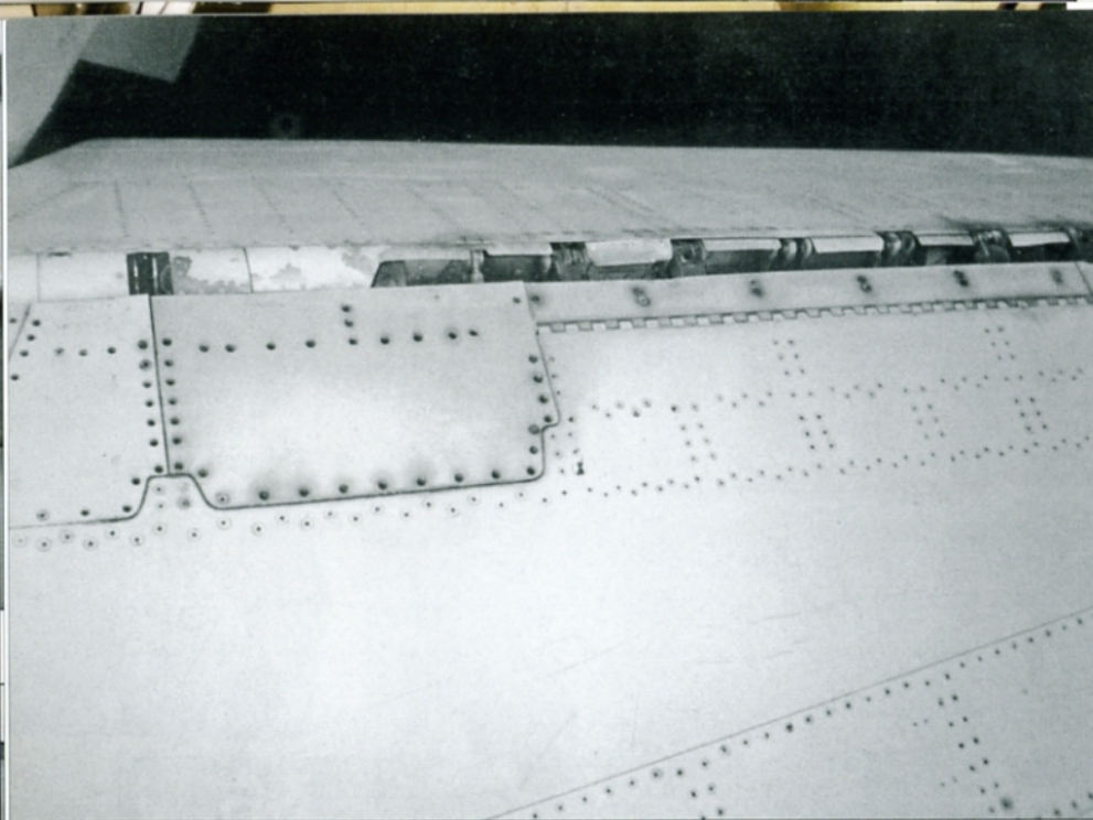
(Above left) The hinges for the flaperons on an Su-27 Flanker-B, viewed from the top. (Sergej F. Sergejev)
