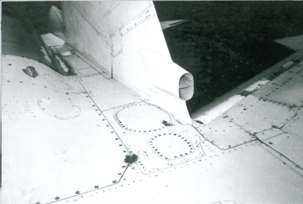
An air intake for the oil cooler is positioned on the root of both fins. The air intake remained unchanged through the production cycle of the Su-27 Flanker-B and Su-27UB Flanker-C trainer. ( Sergej F. Sergejev )
